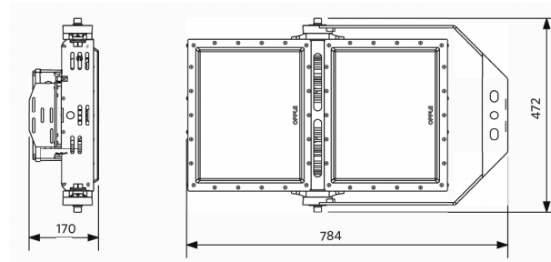
LEDfloodHO-P-620W (+MountingKit-2Mod)
