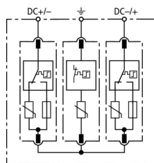
Basic circuit diagram DG M YPV SCI 1200
