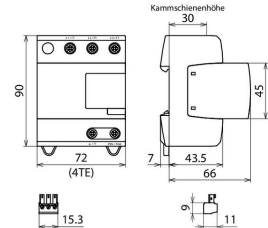
Dimension drawing DV M2 TNC 255 FM
