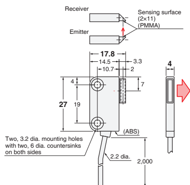
49-B E32-T16JR 2M (Free Cutting)
