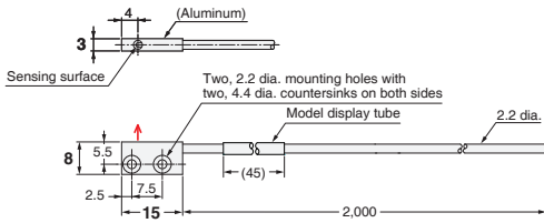
15-B E32-T15YR 2M (Free Cutting)
