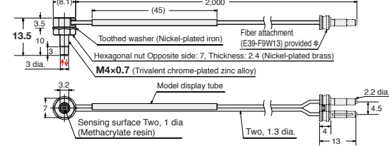
99-E E32-D21N 2M (Free Cutting)
