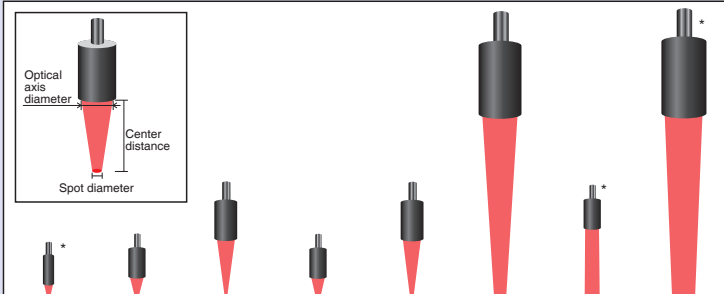
<Map of Spot Diameters and Center Distances> (Unit: mm)
