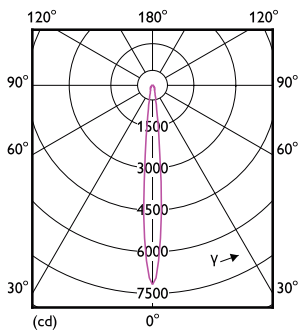
LEDspots 50W G53 AR111 927 8D
