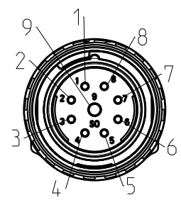
socket face female
