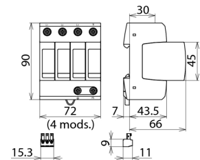
Dimension drawing DG M TT 385/305 FM
