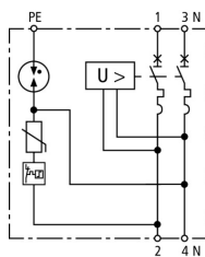
Basic circuit diagram SPD+POP 2 255 C40
