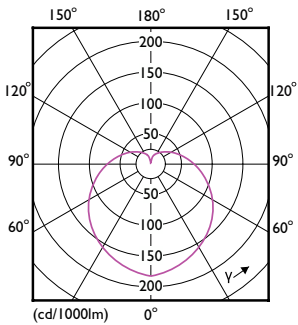
Light Distribution Diagram - LEDbulb ND 4.9-40W A60 E27 827 2CT
