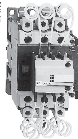
LC1 DPK12••
