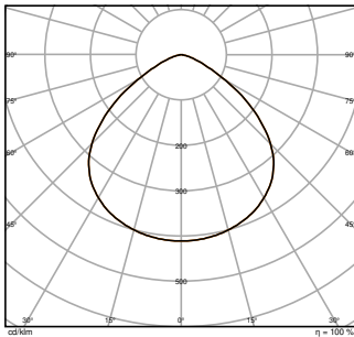
HB P 150W 865 110DEG IP66 PS
