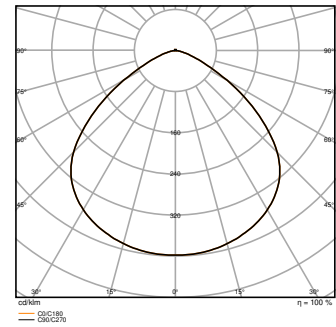
HB P 125W 865 110 DEG IP66 PS
