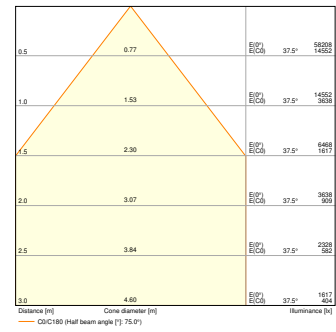
HB P 150W 865 110 DEG IP66 PS - REFRACTOR
