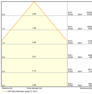
HB P 150W 865 110 DEG IP66 PS - REFLECTOR
