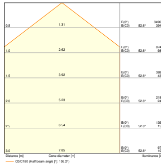
HB P 150W 865 110 DEG IP66 PS set to 125W
