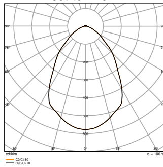
HB P 150W 865 110 DEG IP66 PS - REFRACTOR
