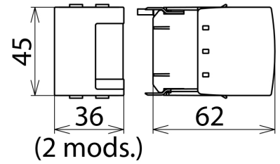
Dimension drawing DGP H MOD 255
