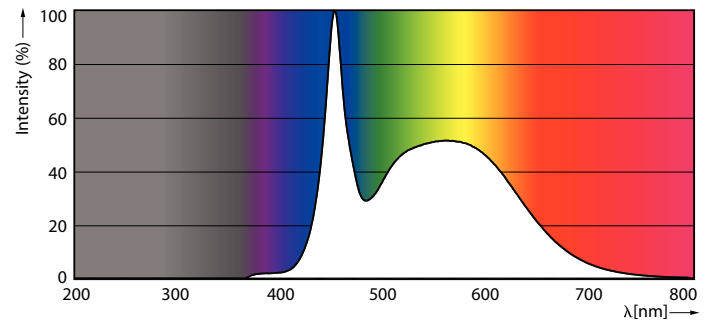
Spectral Power Distribution Colour - CorePro LEDbulb ND 12.5-100W A60 E27 865
