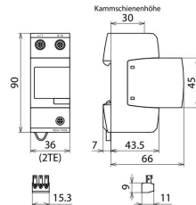
Dimension drawing DV M2 TN 255 FM
