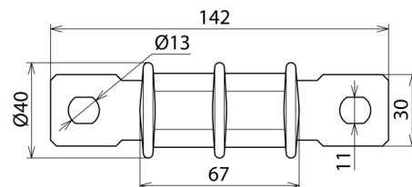
Dimension drawing DSFS
