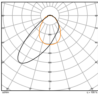
TRUSYS FLEX P 35W 865 WW CL WT
