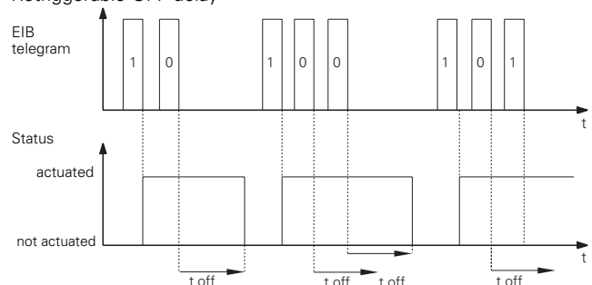
Retriggerable OFF delay
