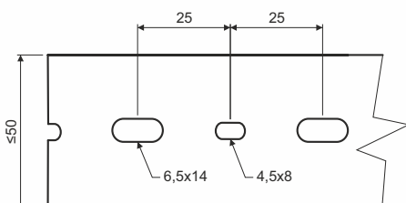
Perforation in one row up to the width of 50 mm.
