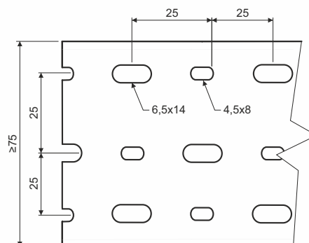
Perforation in three rows above the width of 75 mm.
