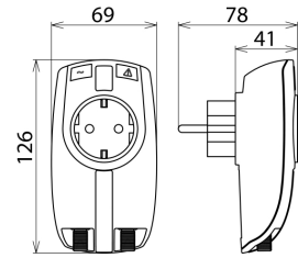
Dimension drawing DPRO 230 TV
