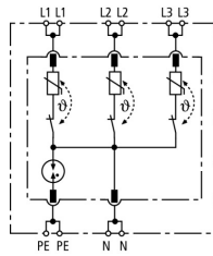
Basic circuit diagram DR M 4P 255
