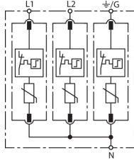
Basic circuit diagram DG MU SPN 240 3W+G
