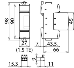
Dimension drawing DG SE DC 550 FM
