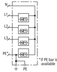
Basic circuit diagram DSH ZP B TT 255
