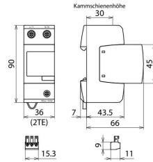
Dimension drawing DV M2 TT 2P 255 FM
