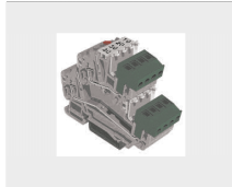
Detail with 5.08 mm female connectors inserted on the two levels and the lug protection covers raised
