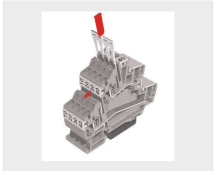
Detail of PTC jumper with DFM500 barriers, CNU/8/51 numbering strips and VPC/VT lug protection covers
