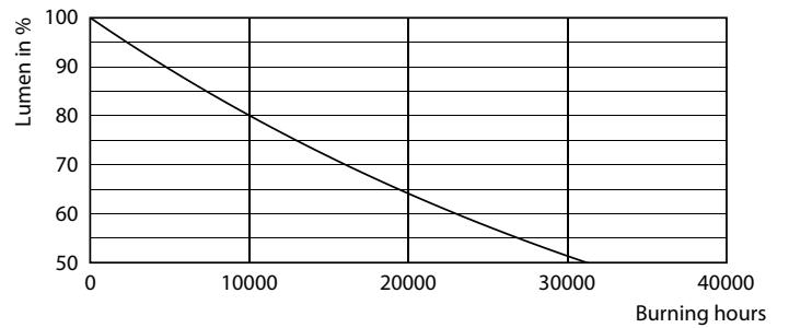
Lumen Maintenance Diagram - MAS VLE LEDBulbD3.4-40W E27 940 A60FR G
