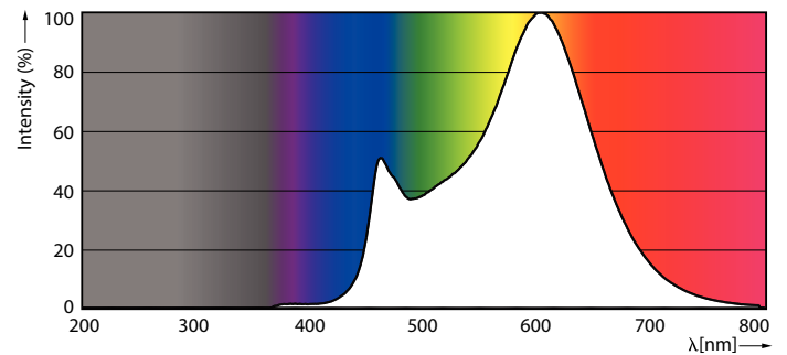
Spectral Power Distribution Colour - CorePro LEDbulb ND 5-40W A60 E27 830
