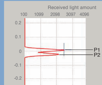
Received Waveform for ZW-series Sensor
