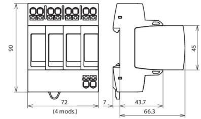
Dimension drawing DG MP TT 275
