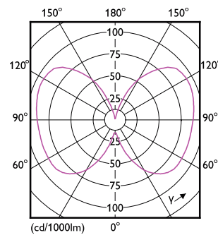
Light Distribution Diagram - MAS LEDBulbND4-60W E27 840 G95 CL G UE
