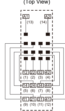
Terminal Arrangement/Internal Connection Diagram (Top View)
