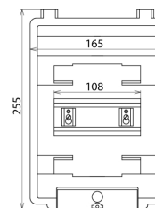
Dimension drawing IGA 6 IP54
