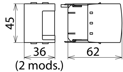
Dimension drawing DB M MOD 255
