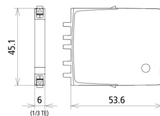
Dimension drawing BCO MOD ML2 BE 24
