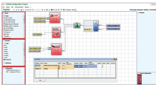
Text visualization
