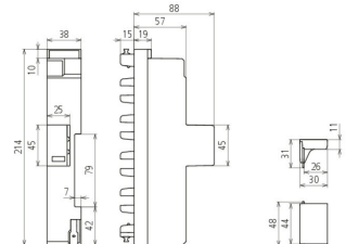
Dimension drawing DSH ZP B2 TNS 255
