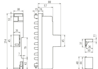
Dimension drawing DSH ZP B2 TNC 255
