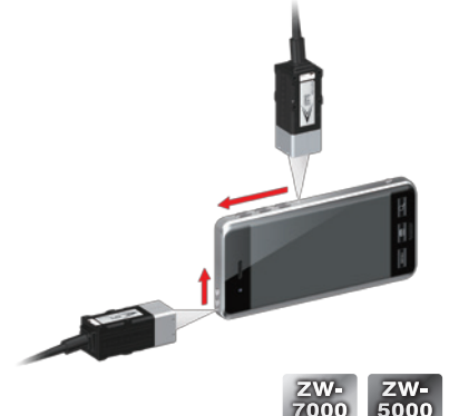
Level difference measurement between buttons and case
