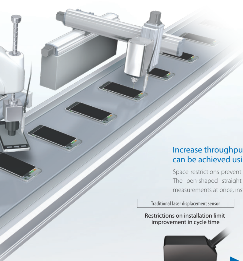
White light confocal displacement sensor
