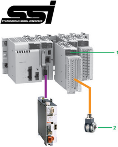
Modicon X80 module platform with Modicon M340 processor
