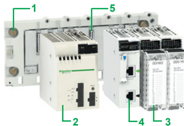
Typical basic assembly with Modicon X80 I/O modules
