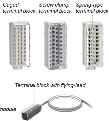
Accessories for connecting 20-pin modules
