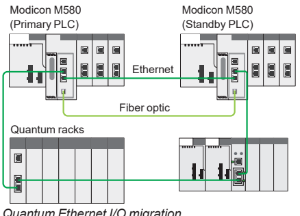
Quantum Ethernet I/O migration
