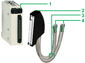
Preassembled cordset with 40-way connector and two ends with flying leads
