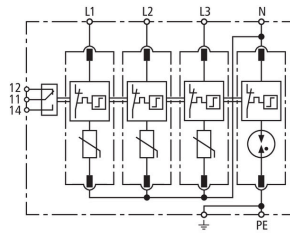
Basic circuit diagram DG M TT 320 FM
