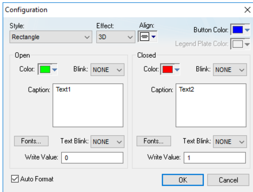
Configuration dialog
