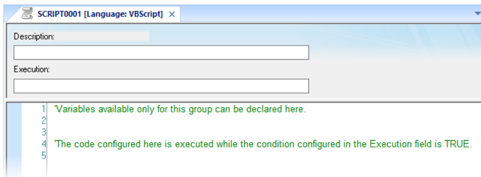
Script worksheet
