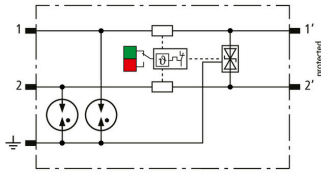
Basic circuit diagram BCO ML2 BE HF 5
