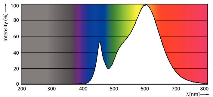
Spectral Power Distribution Colour - CorePro LEDbulb ND 4.9-40W A60 E27 830
