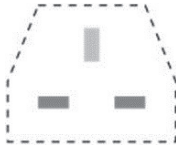
British Standard 13A 2P+E (250V)
